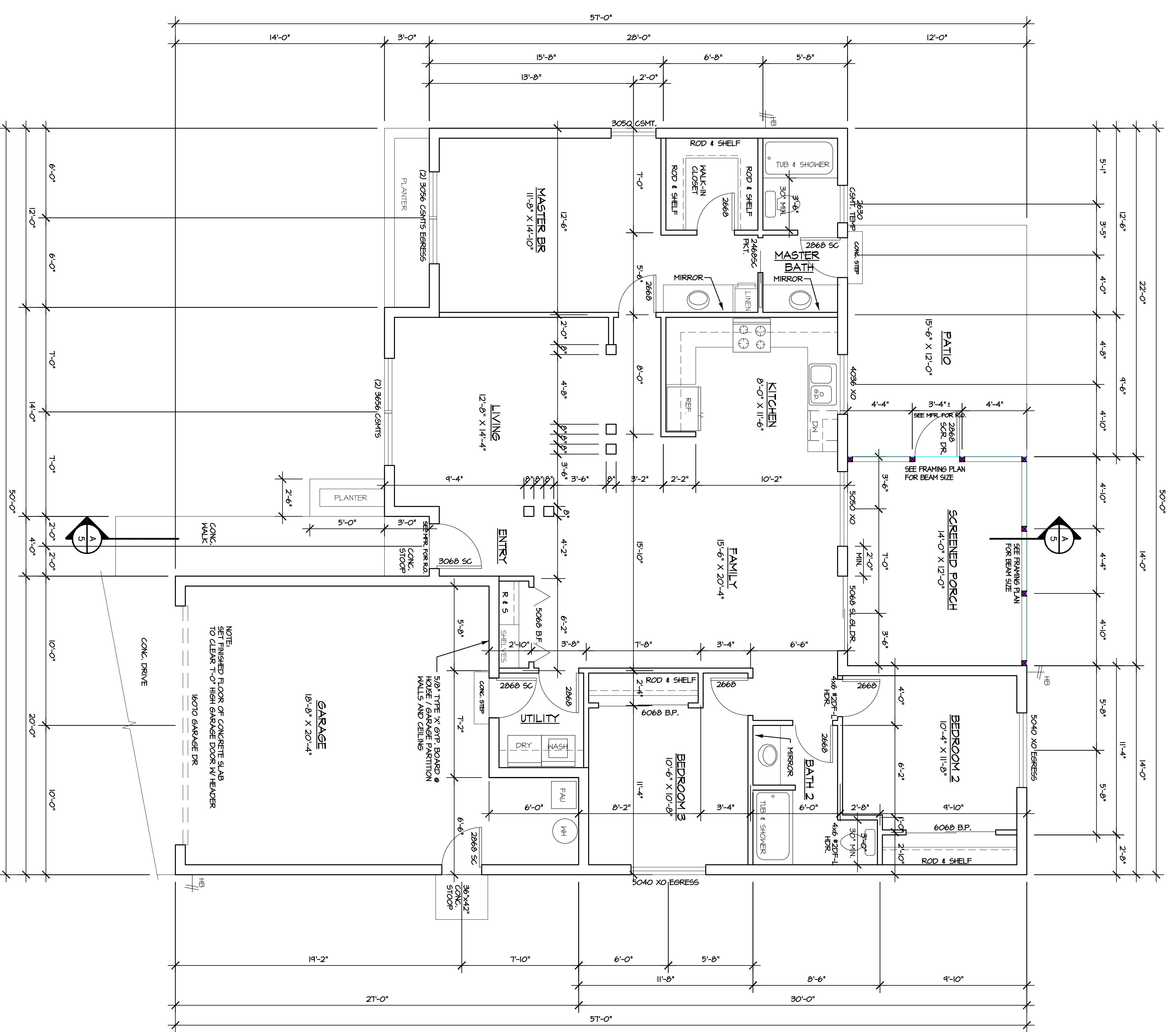
1 FLOOR PLAN 1/4" = 1'-0"
